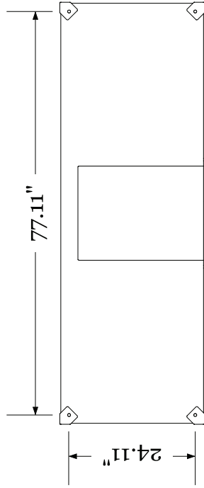
MOUNTING HOLE PATTERN DIMENSION (27" x 80" INSIDE BED PAN DIMENSION)
