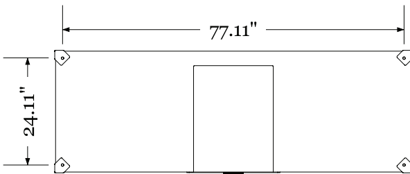
MOUNTING HOLE PATTERN DIMENSION (27" x 80" INSIDE BED PAN DIMENSION)
