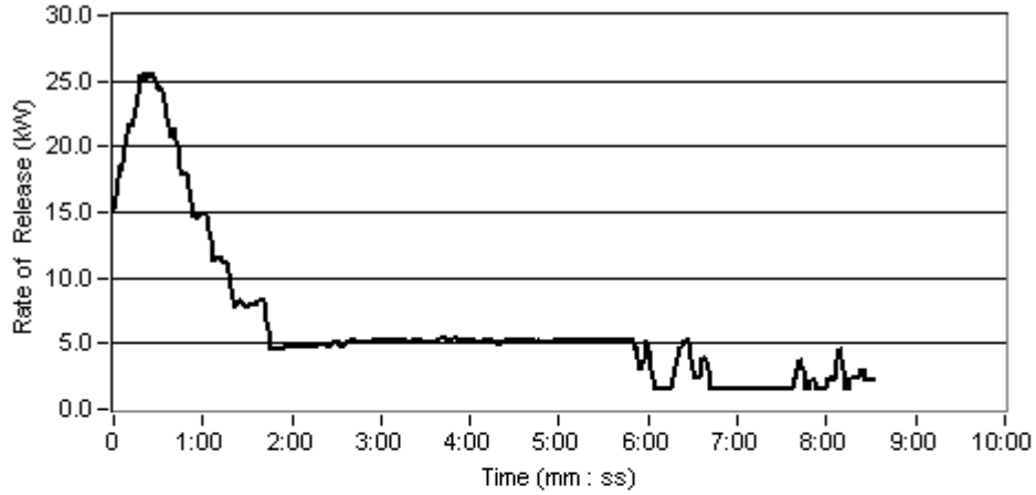
Rate of Heat Release
